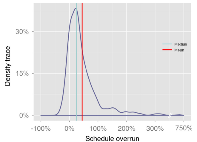
Fig. 5. Density trace of schedule slippage ( N=239 ) with the median and mean.
